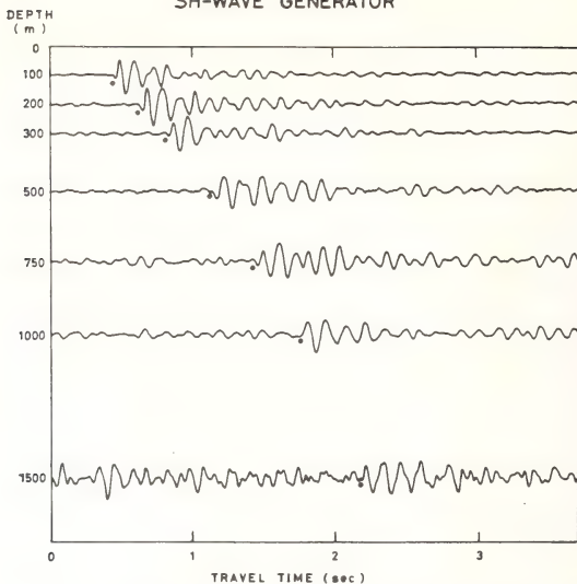
Fig. 3 Resynthesized records of the SH-wave generator. Solid circles show the onset of S waves.
